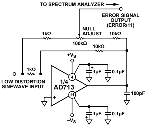
Figure 36. THD Test Circuit
