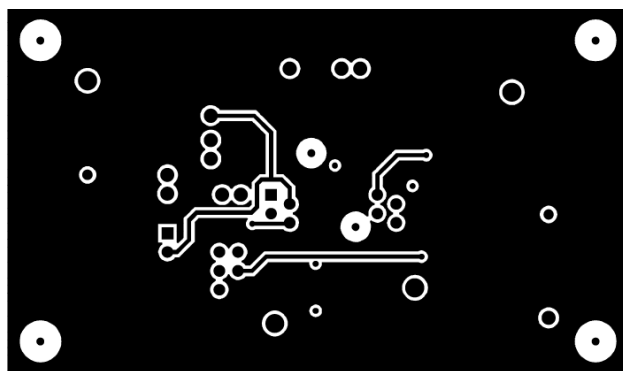
Figure 35. AD737 Evaluation Board—Secondary-Side Copper
