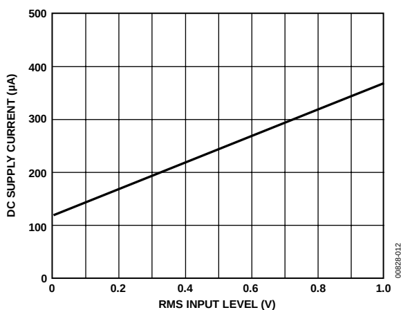
Figure 12. DC Supply Current vs. RMS Input Level
