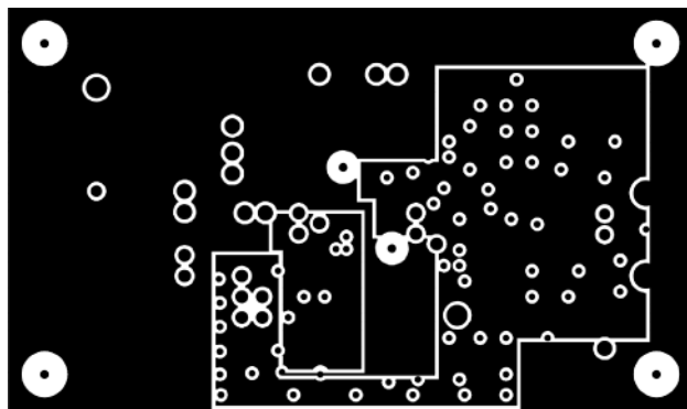
Figure 36. AD737 Evaluation Board—Internal Power Plane
