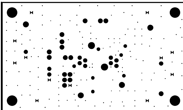
Figure 37. AD737 Evaluation Board—Internal Ground Plane
