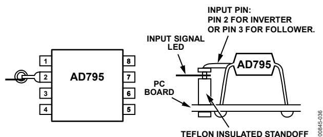
Figure 36. Input Pin to Insulating Standoff
