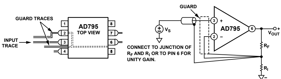
Figure 35. Guard Scheme—Follower
