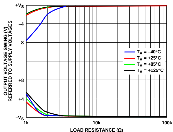
Figure 20. Output Voltage Swing vs. R_L and Temperature, V_S = \pm 15\text{ V}
