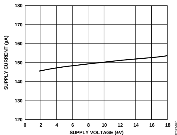
Figure 22. Supply Current Per Channel vs. Dual Supply Voltage, V_{IN} = 0\text{ V}
