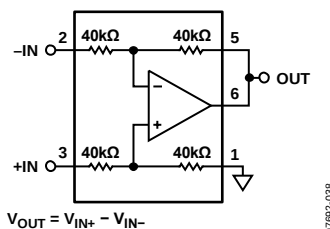
Figure 42. Difference Amplifier, Gain = 1
