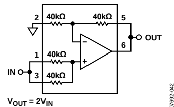
Figure 46. Noninverting Amplifier, Gain = 2
