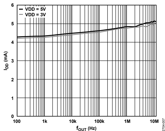
Figure 7. Typical I_{DD} vs. f_{OUT} for f_{MCLK} = 25\text{ MHz}
