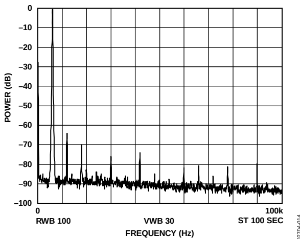
Figure 14. Power vs. Frequency, f_{MCLK} = 10 MHz, f_{OUT} = 2.4 kHz, Frequency Word = 0x000FBA9
