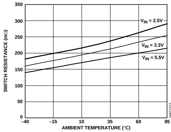
Figure 11. Switch Resistance vs. Ambient Temperature
