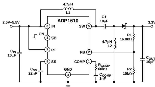
Figure 30. 3.3 V DC-DC Converter
