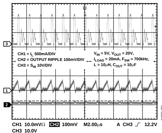
Figure 21. Switching Waveform in Discontinuous Conduction
