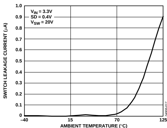
Figure 17. Switch Leakage Current vs. Ambient Temperature
