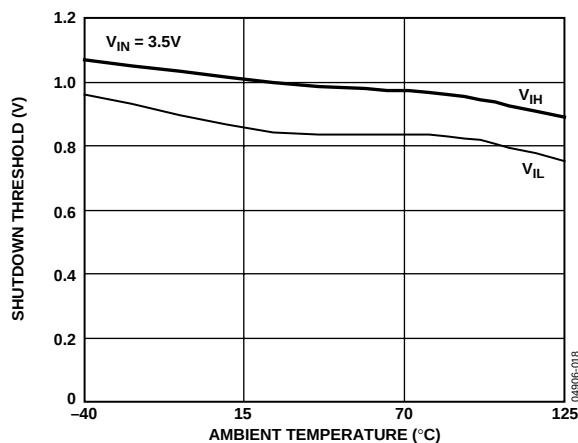
Figure 18. Shutdown Threshold vs. Ambient Temperature
