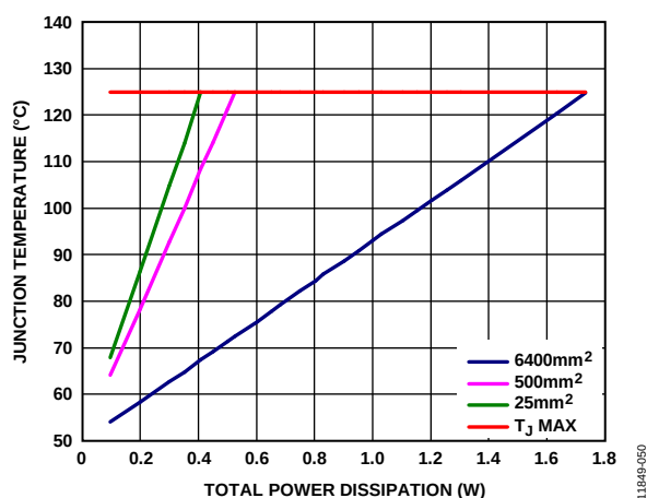
Figure 53. LFCSP, T_A = 50^{\circ}\text{C}
