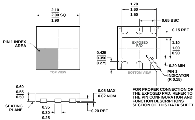
Figure 67. 6-Lead Lead Frame Chip Scale Package [LFCSP_UD] 2.00 mm × 2.00 mm Body, Ultra Thin, Dual Lead (CP-6-3) Dimensions shown in millimeters
