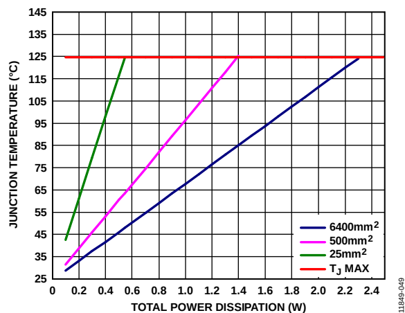
Figure 52. LFCSP, T_A = 25^{\circ}\text{C}
