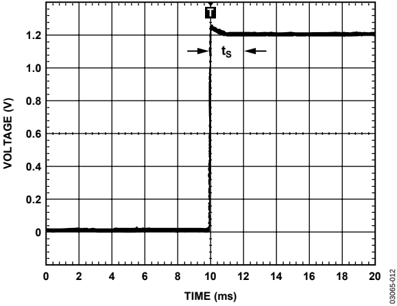
Figure 10. Settling Time
