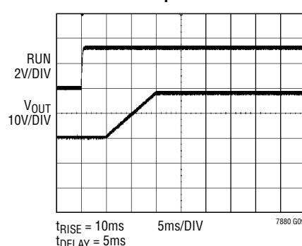
Soft-Start Ramp
