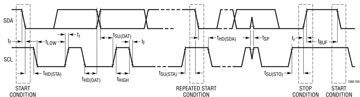
Figure 5. Timing Diagram
