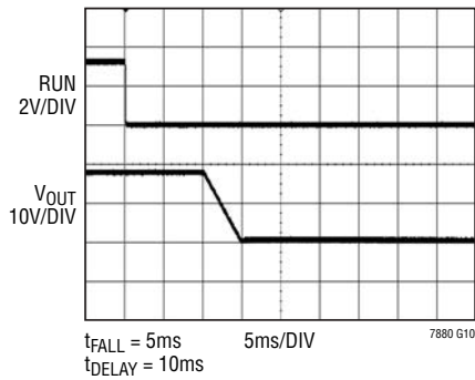
Soft-Off Ramp
