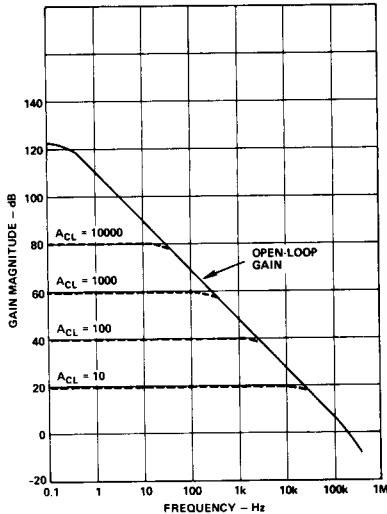
Small-Signal Gain vs. Frequency
