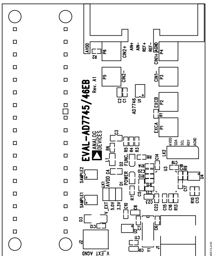
Figure 15. Evaluation Board Layout, Silkscreen
