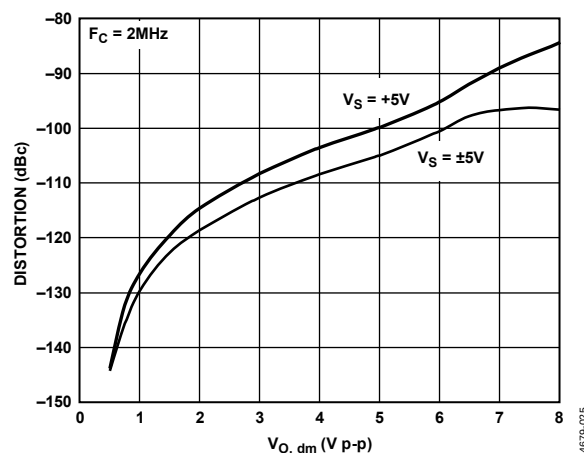
Figure 29. Third Harmonic Distortion vs. Output Amplitude
