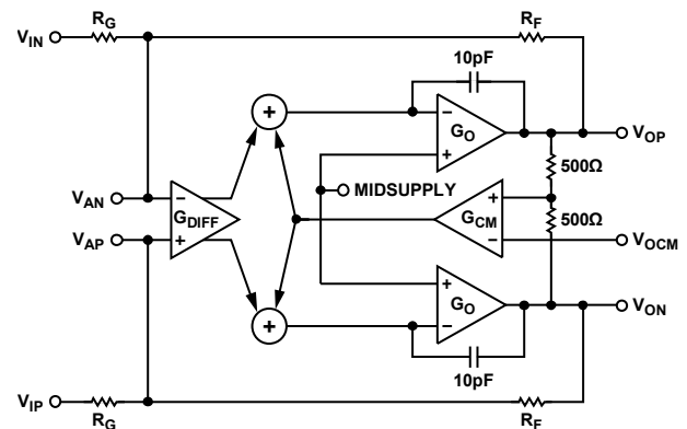
Figure 60. Block Diagram
