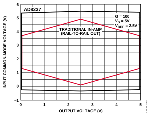
Figure 2. Input Common-Mode Voltage vs. Output Voltage, +V_S = 5\text{ V} , G = 100
