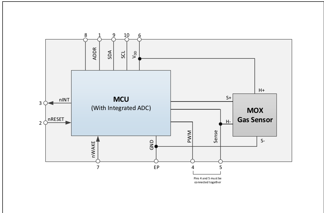
Figure 2: CCS811 Block Diagram
