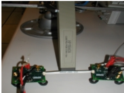
FIGURE 1. Test Set-up
