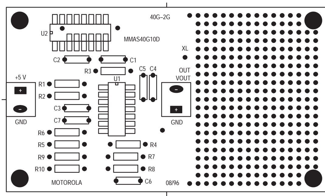
Figure 5. Silk Screen
