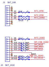
SHIELD BOARD ARDUINO HEADER
