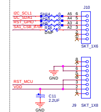
SHIELD BOARD ARDUINO HEADER
