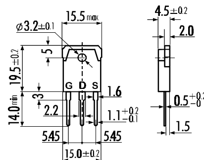
TO-3P
