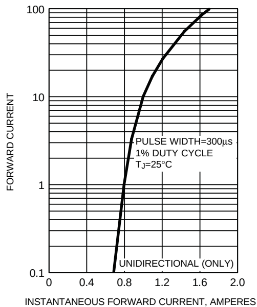
FIG. 11 - INSTANTANEOUS FORWARD VOLTAGE CHARACTERISTICS CURVE
