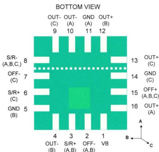
HMC1053 Pinout
