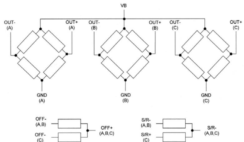
HMC1053 Circuit Diagram
