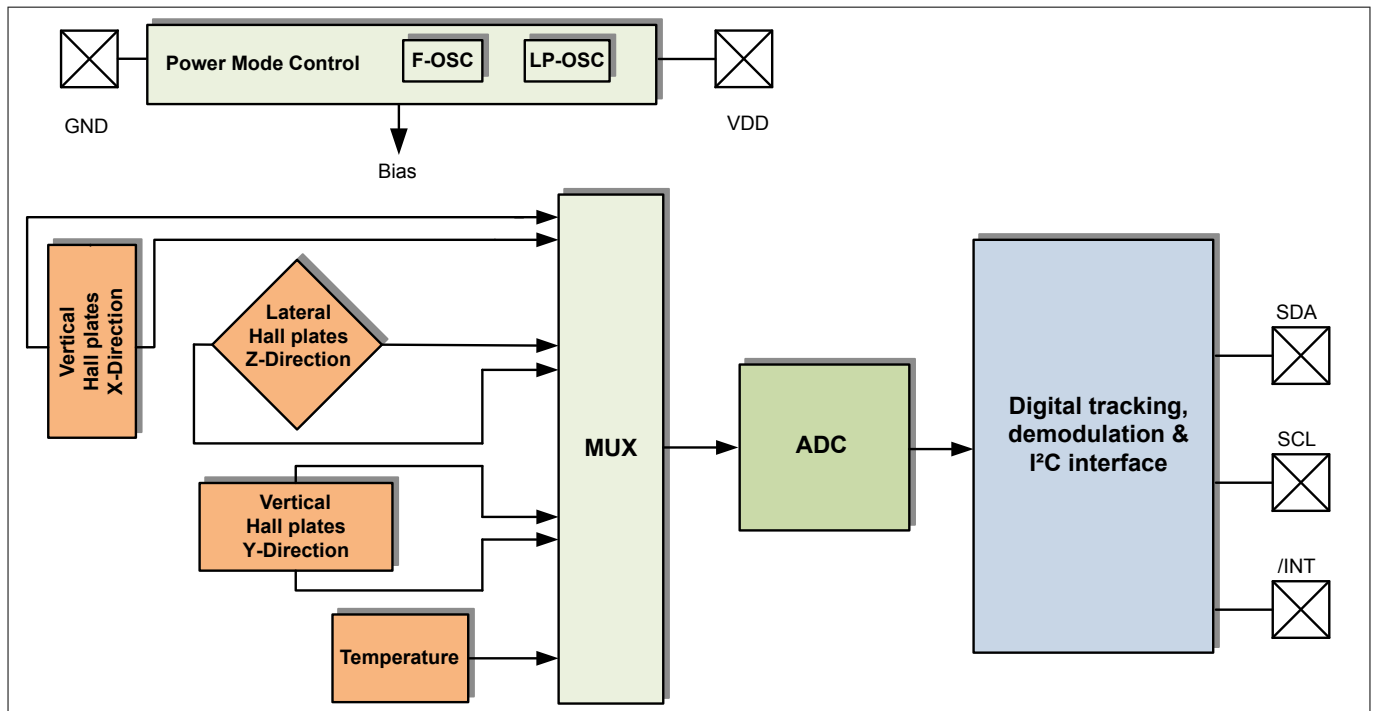
Figure 1 Block diagram
