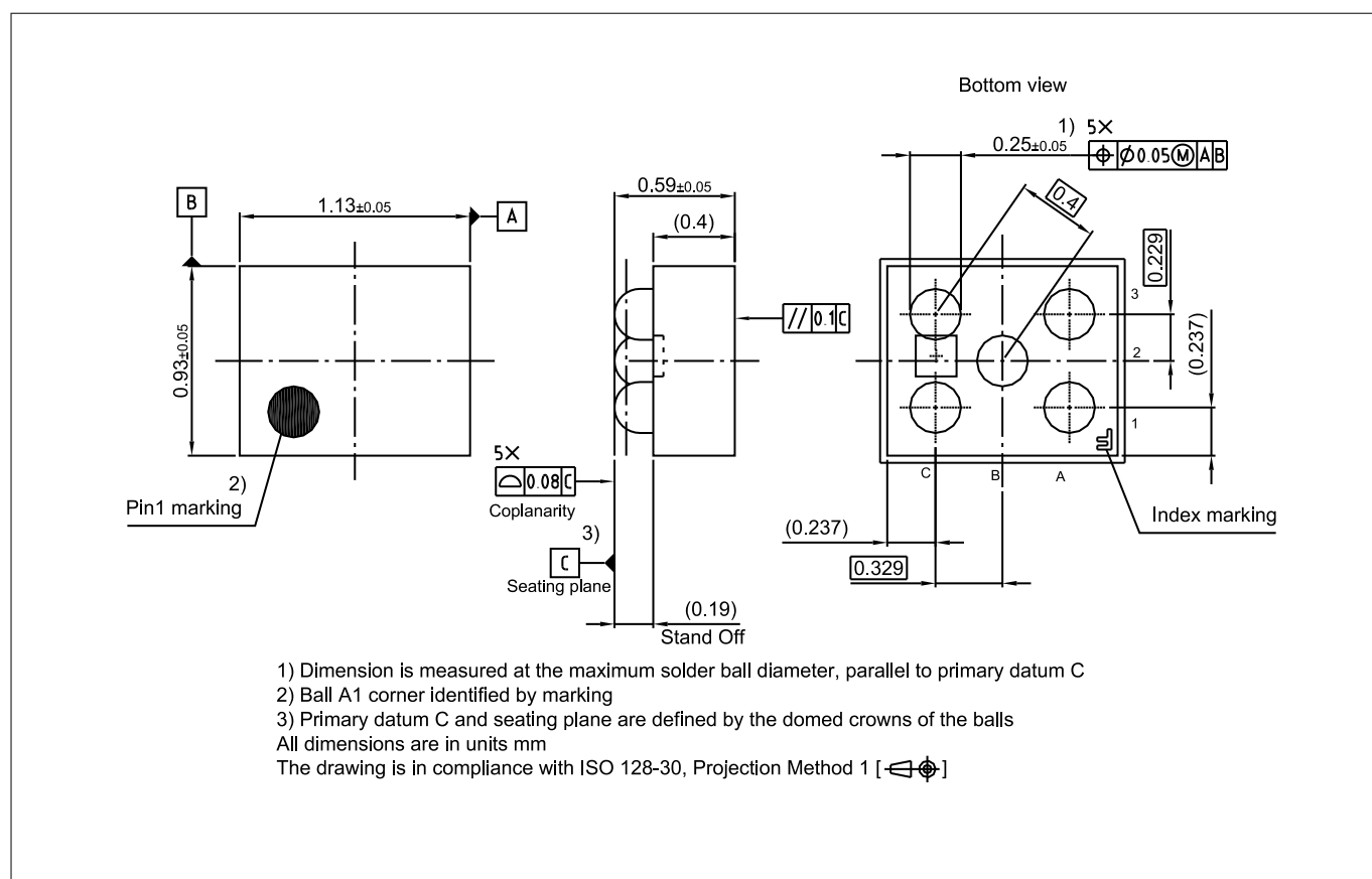
Figure 10 Package outlines
