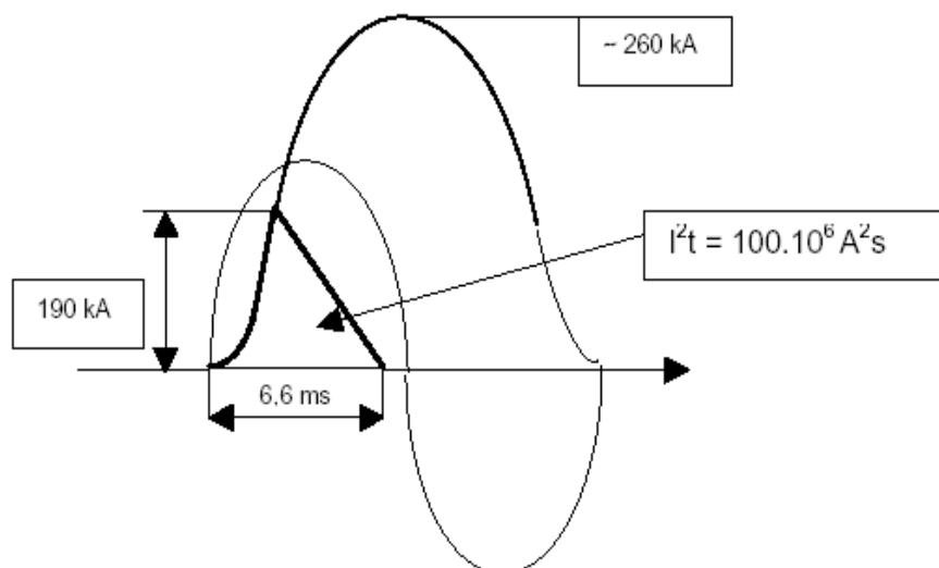
Fig. 2 Typical semiconductor load at fuse switching.
