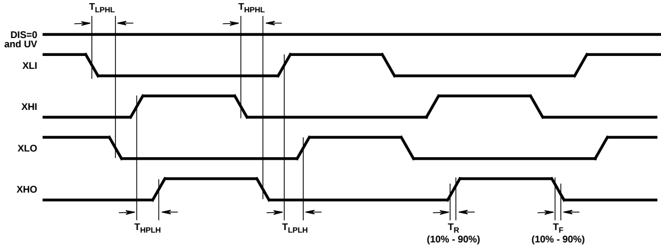
FIGURE 1. INDEPENDENT MODE
