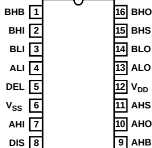
HIP4082 (PDIP, SOIC) TOP VIEW
