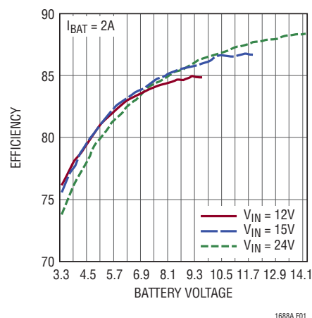
Figure 1. LT3652HV Efficiency
