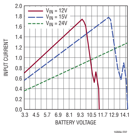
Figure 2. 2A Charge Current
