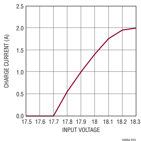
Figure 3. Charge Current vs Input Voltage
