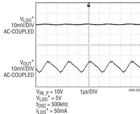
LDO+ Rejection of V_{OUT^+} Ripple
