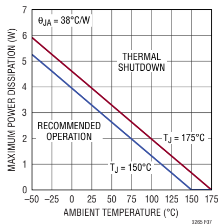
Figure 7. Maximum Power Dissipation vs Ambient Temperature
