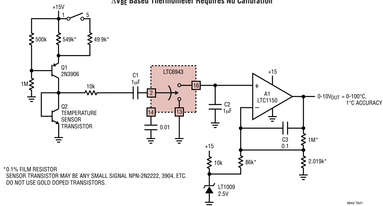
\Delta V_{BE} Based Thermometer Requires No Calibration
