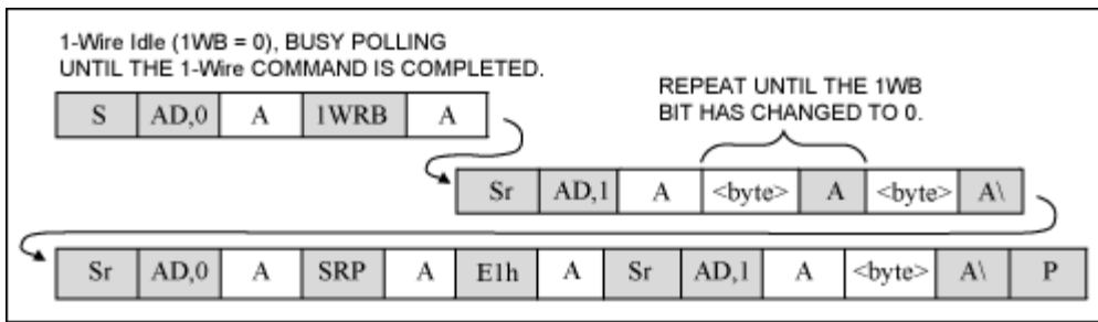
Figure 10. 1-Wire Read Byte. Reads a byte from the 1-Wire network. Poll the Status register until the 1WB bit has changed from 1 to 0. Then set the read pointer to the Read Data register (code E1h) and access the device again to read the data byte obtained from the 1-Wire network.
