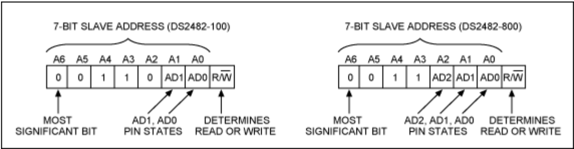
Figure 2. DS2482 I 2 C slave addresses.
