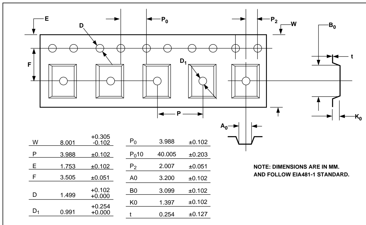
Tape-and-Reel Information
