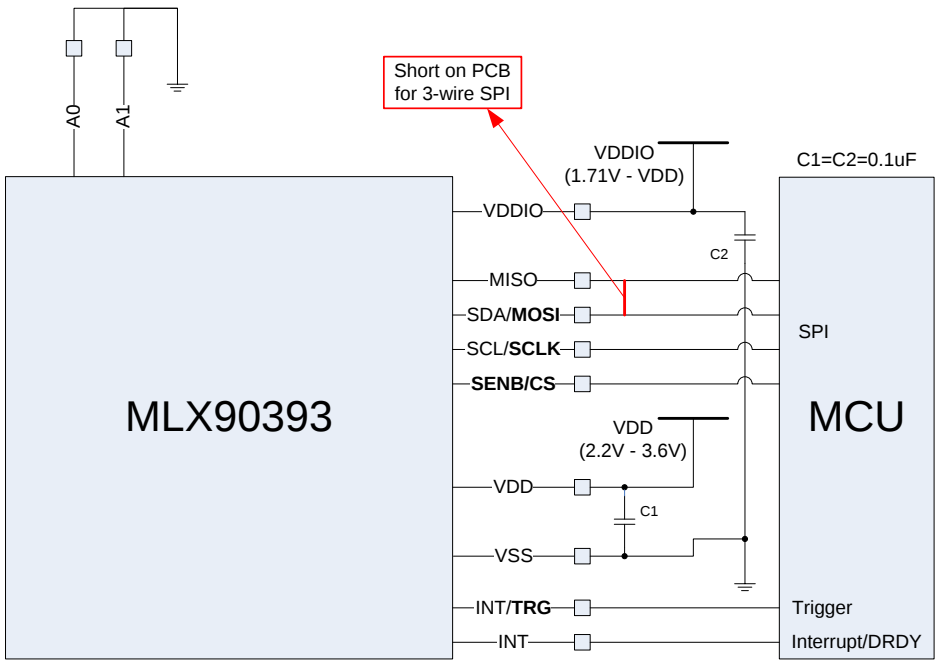
Figure 24: 3/4wire SPI recommended schematic
