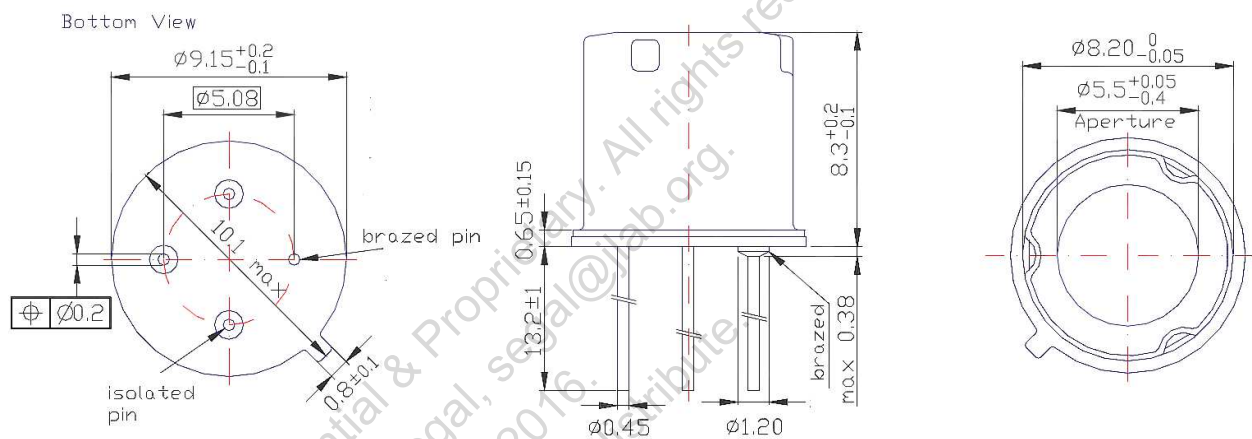
Figure 44: MLX90614xCH package
