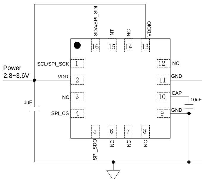
<Top View> SPI Single Supply Connection
