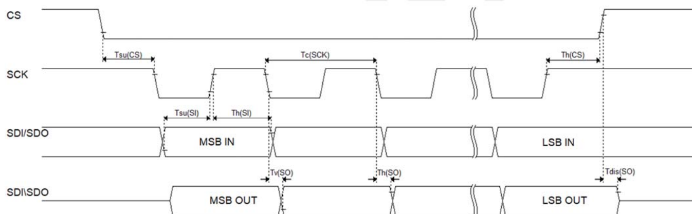
Timing Definition
