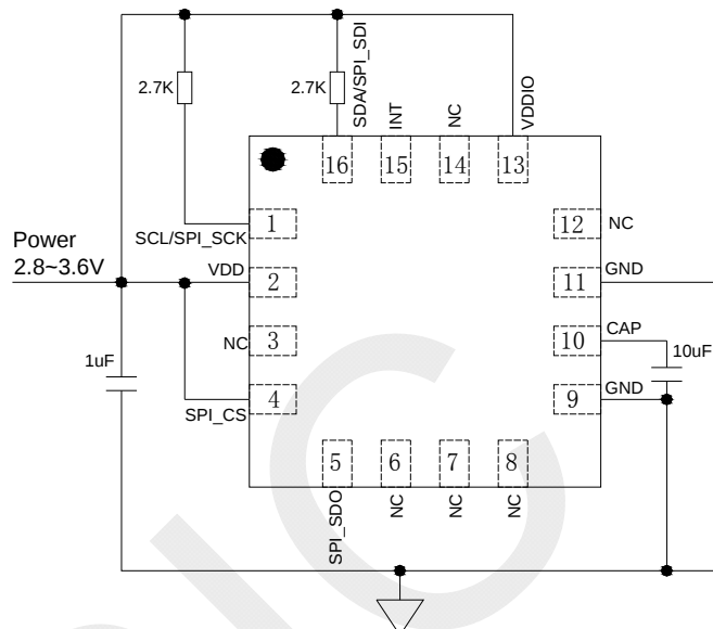
<Top View> I 2 C Single Supply Connection
