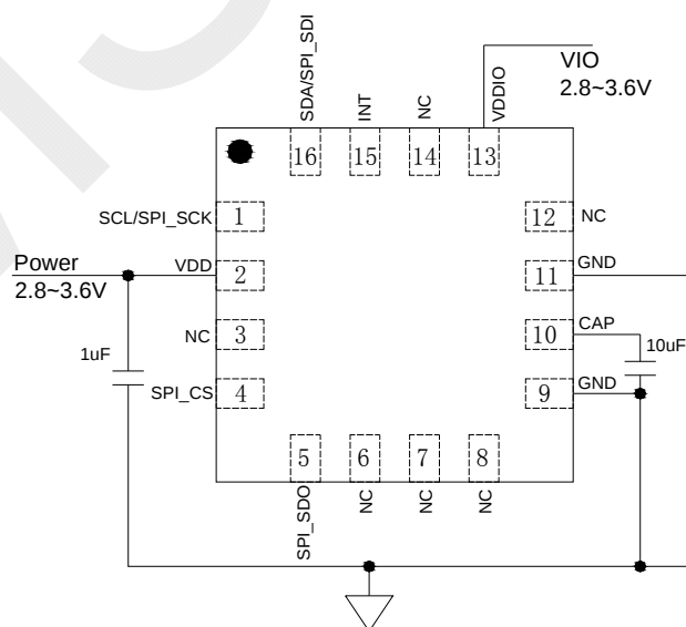
<Top View> SPI Dual Supply Connection
