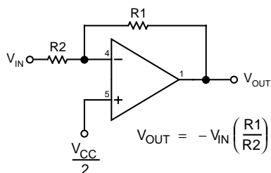
Figure 2. Inverting Amplifier
