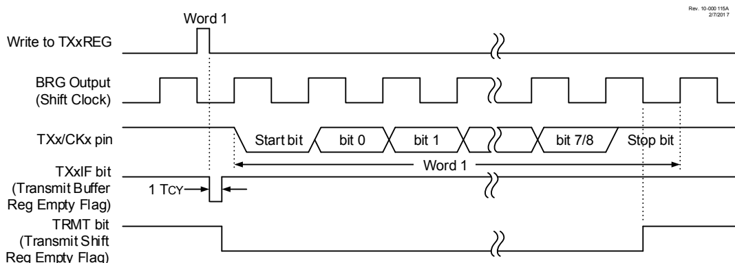
Figure 36-11. Synchronous Transmission
