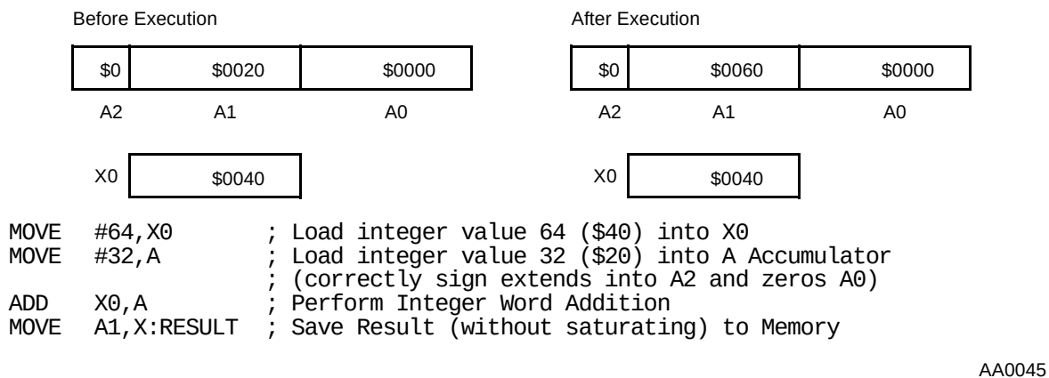
Figure 3-9. Word-Sized Integer Addition Example
