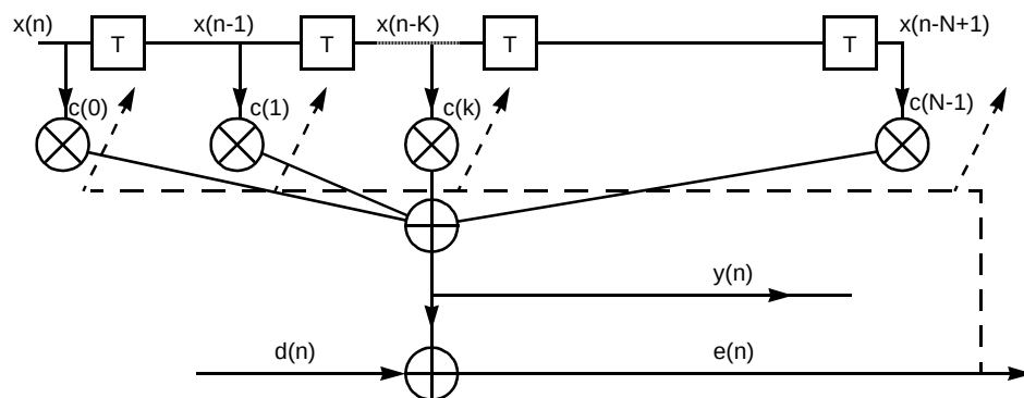
Figure B-2. LMS Adaptive Filter Graphic Representation
