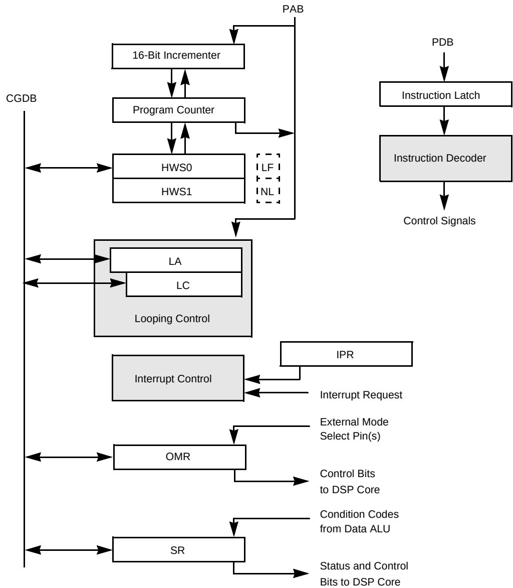
Figure 5-1. Program Controller Block Diagram
