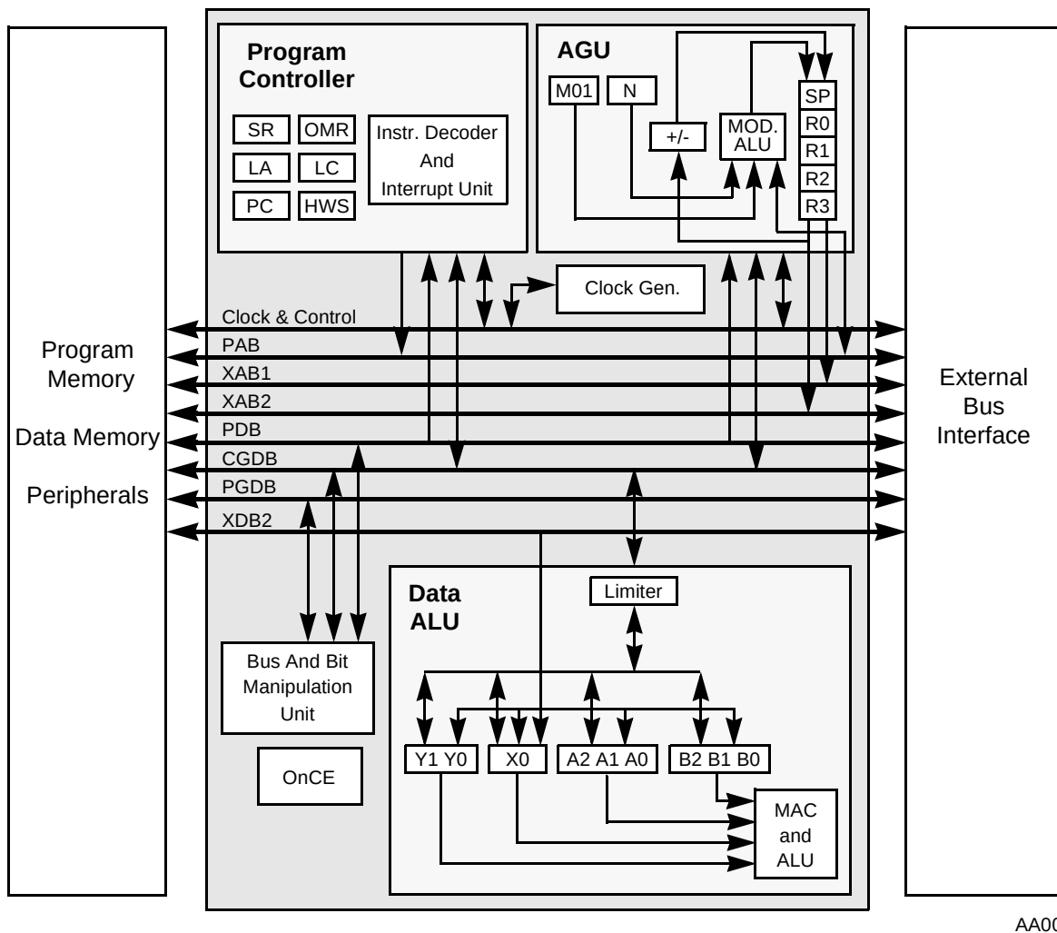
Figure 1-2. DSP56800 Core Block Diagram
