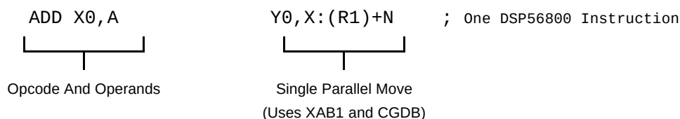
Figure 6-1. Single Parallel Move
