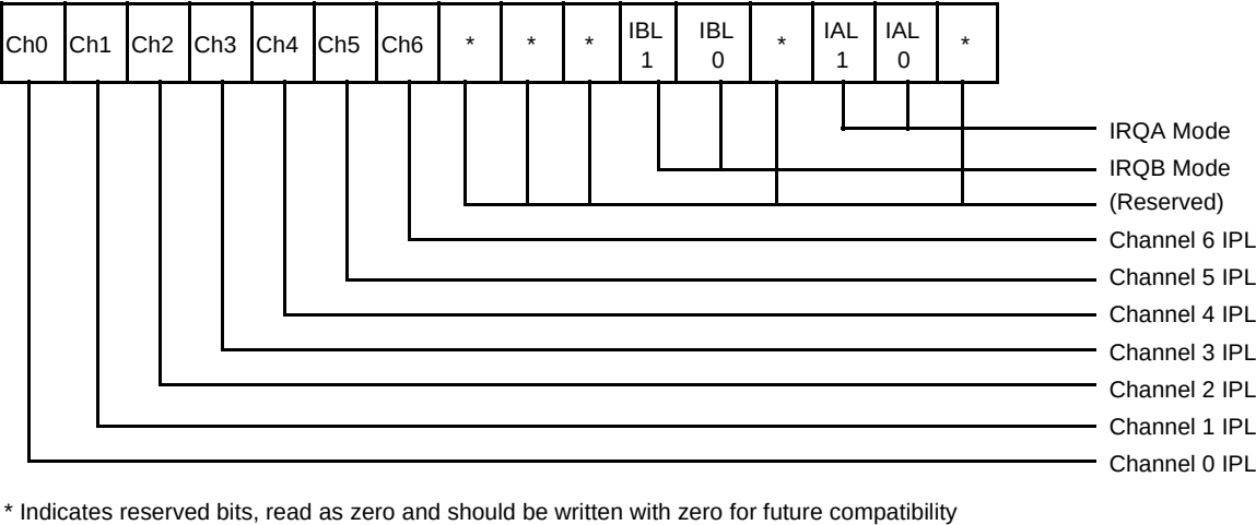
Figure 7-2. Example Interrupt Priority Register
