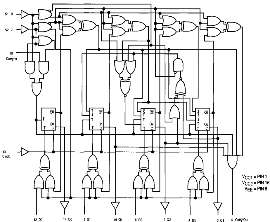
LOGIC DIAGRAM
