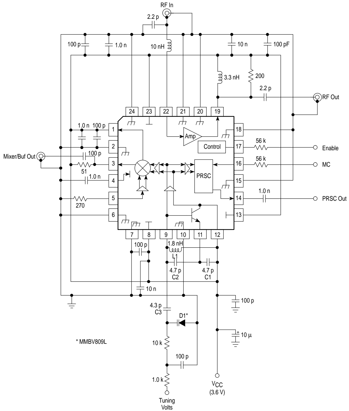
Figure 8. Applications Circuit
