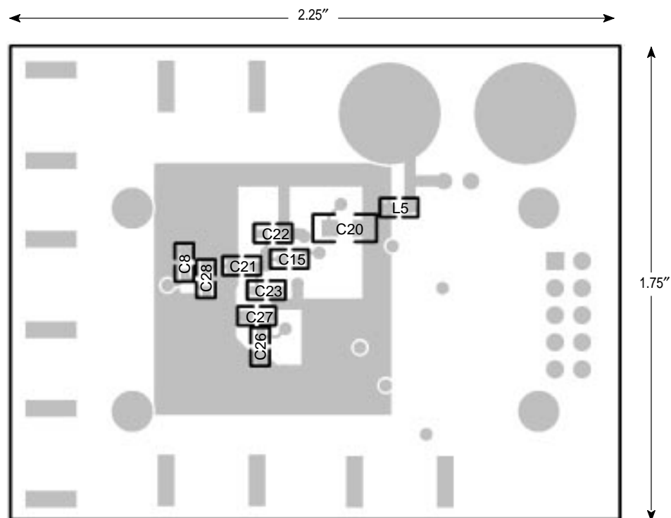
Figure 12. MC13146 Evaluation PCB Solder Side
