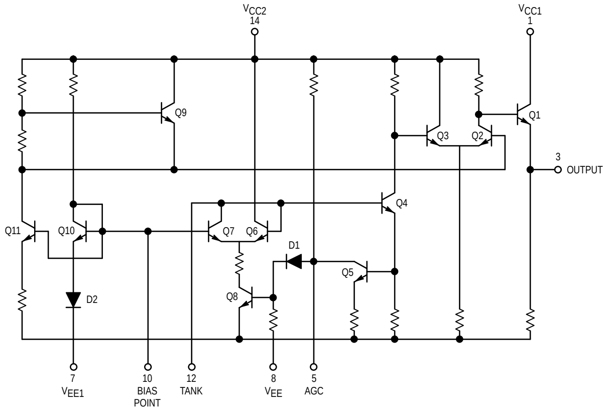
Figure 1. Circuit Schematic
