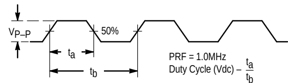
Figure 3. Test Circuit and Waveforms
