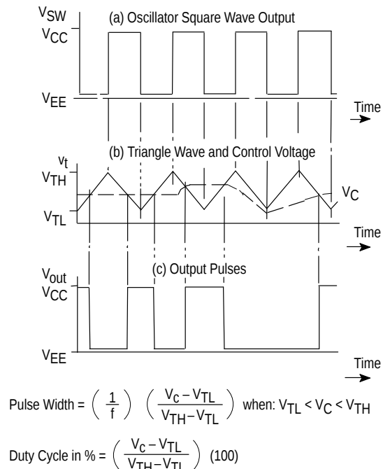
Figure 11. Pulse Width Modulator Schematic and Waveforms
