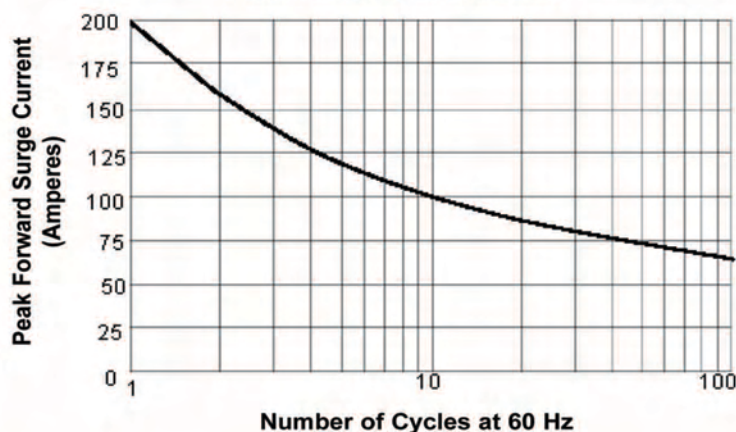
Peak Forward Surge Current
