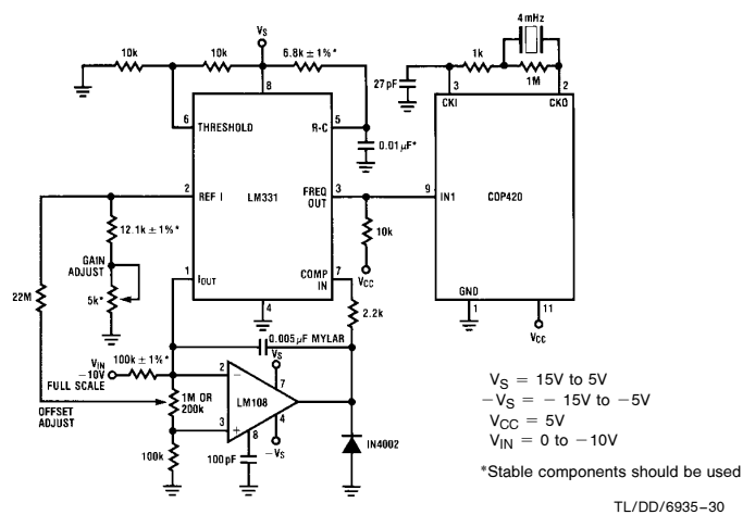
FIGURE 21. A to D with Precision Voltage to Frequency Converter
