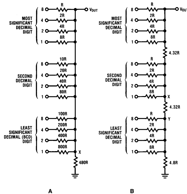
FIGURE 27. 8421 BCD Ladders
