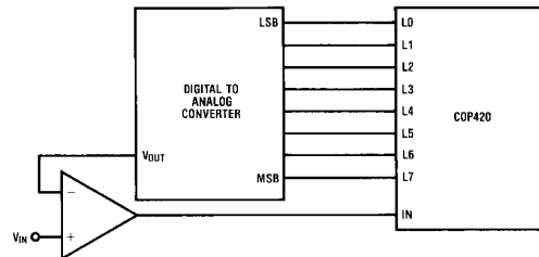
FIGURE 23A. Basic Parallel Implementation
