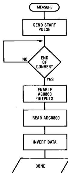
FIGURE 30B. ADC0800 Interface Flow
