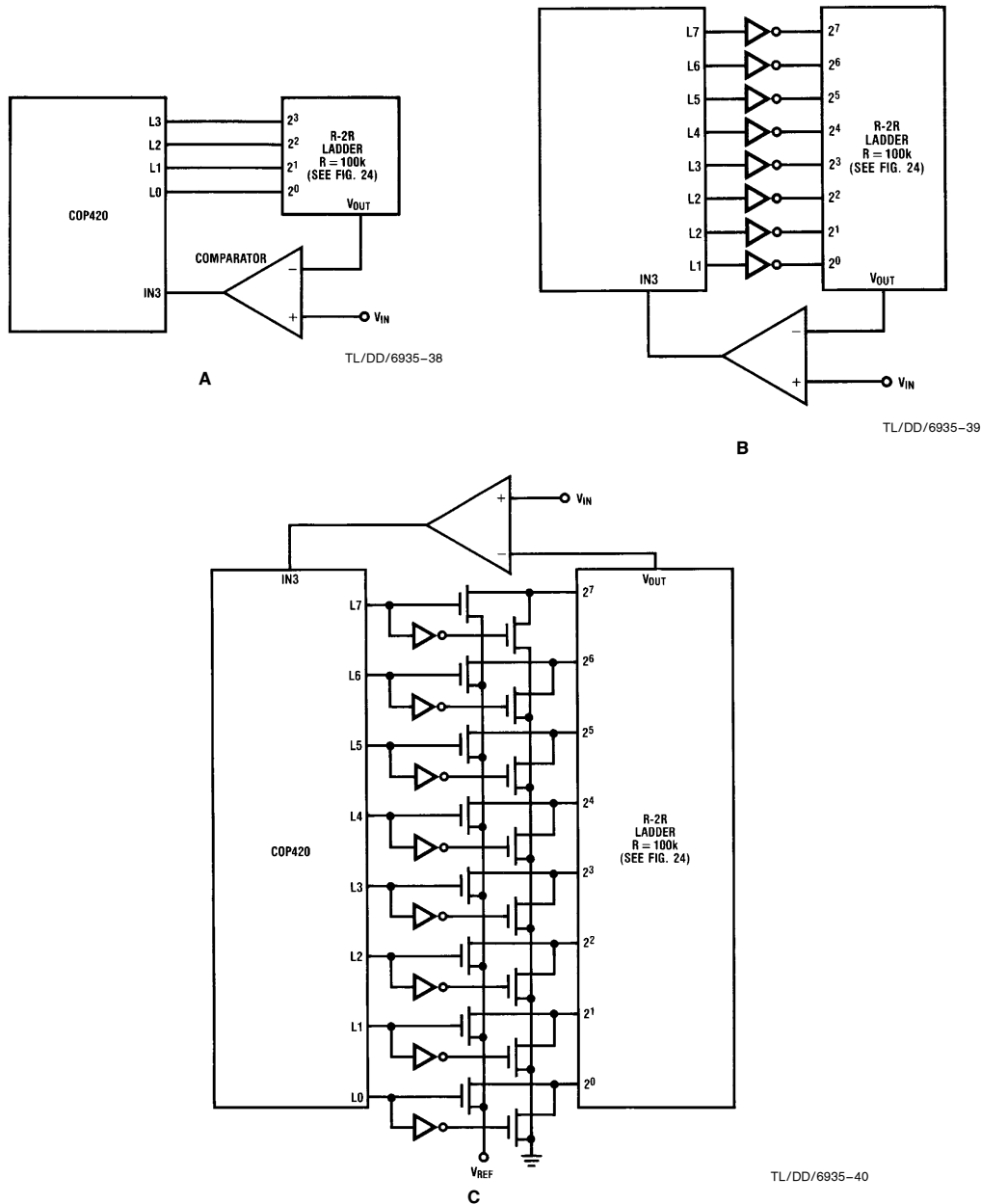
FIGURE 28. Interfaces to Ladder Networks
