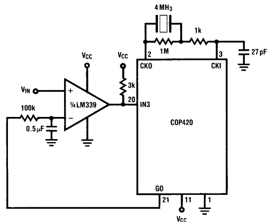
V_{CC} = +5V FIGURE 1. Basic Capacitor Charge Technique
