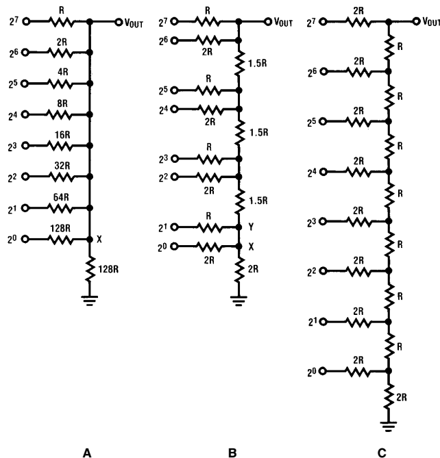
FIGURE 26. Binary Ladders
