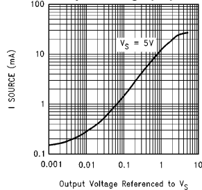
Sourcing Current vs Output Voltage (5V)
