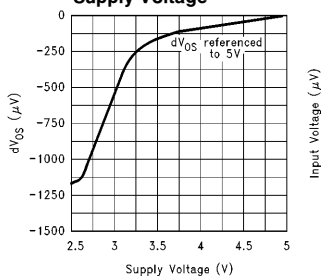
dVOS vs Supply Voltage
