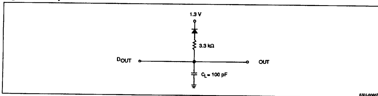
Figure 1. Output Load
