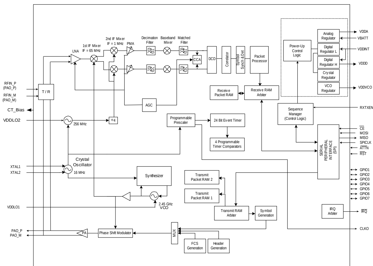
Figure 1. 802.15.4 Modem Simplified Block Diagram
