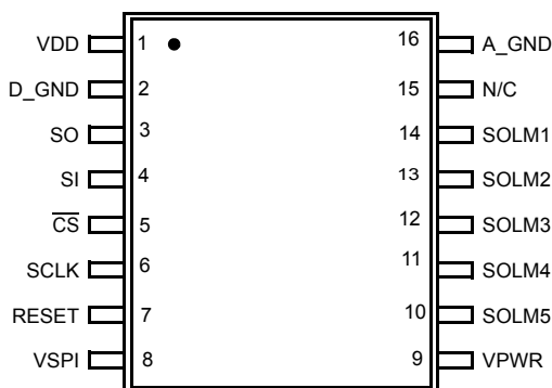
Figure 3. 33811 Pin Connections
