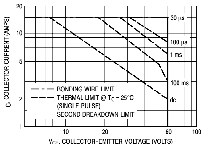
Figure 12. Forward Bias Safe Operating Area 2N3055A
