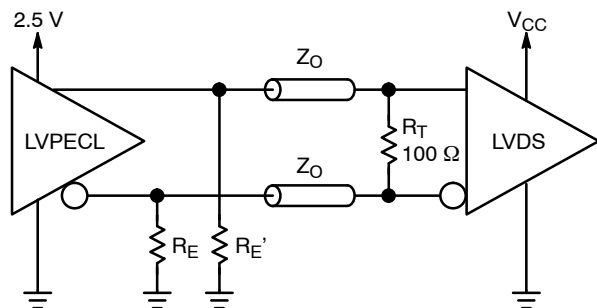
Figure 8. Interfacing 2.5 V LVPECL to LVDS with External 100 \Omega Termination Resistor
