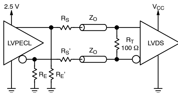
Figure 11. Interfacing 2.5 V LVPECL to LVDS with Series R_S and External 100 \Omega Termination Resistor
