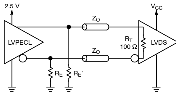
Figure 9. Interfacing 2.5 V LVPECL to LVDS with Internal 100 \Omega Termination Resistor
