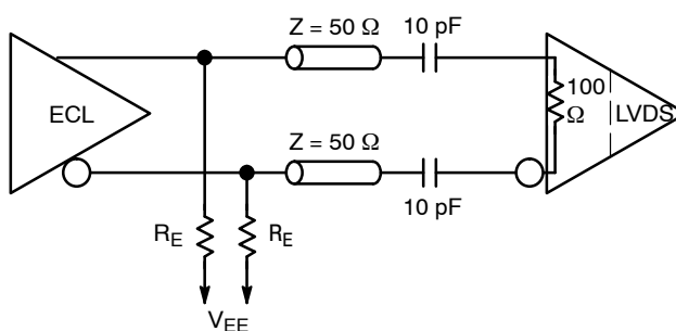
Figure 5. Capacitive Coupling ECL to LVDS
