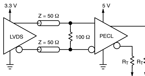
Figure 20. Interfacing LVDS to PECL
