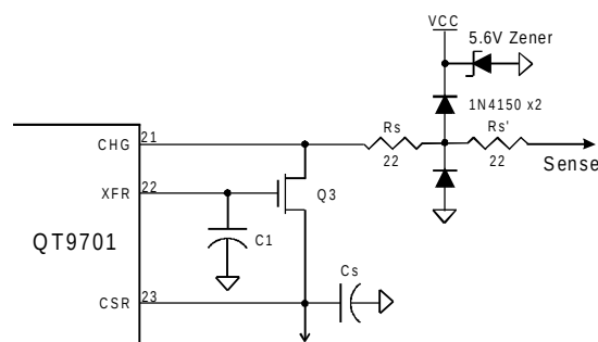
FIGURE 14-1 Recommended ESD Network
