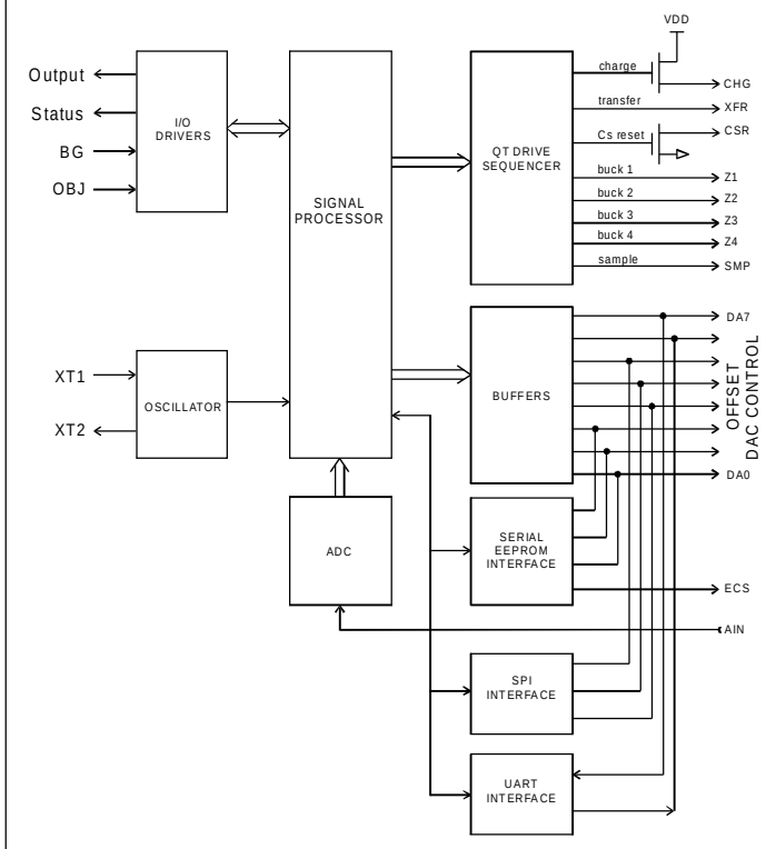
FIGURE 1-1 BLOCK DIAGRAM
