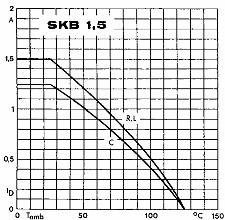
Fig. 1 Rated output current vs. ambient temperature
